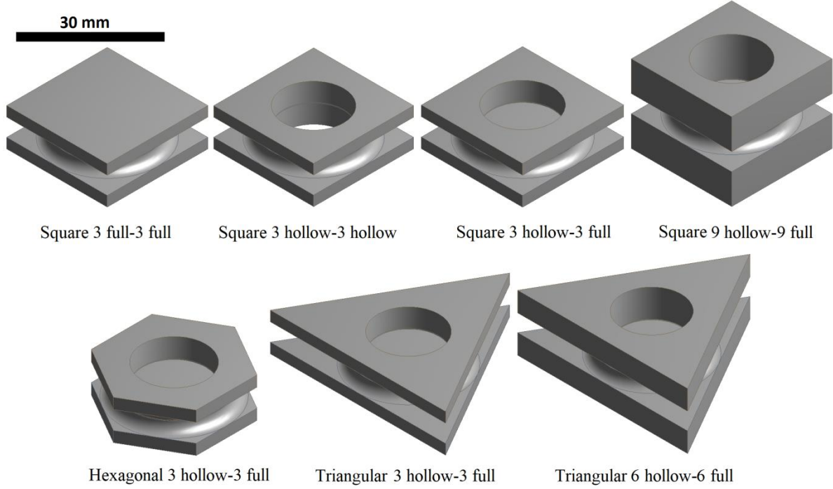
Fig. 2. Schematics of different types of specimens.
